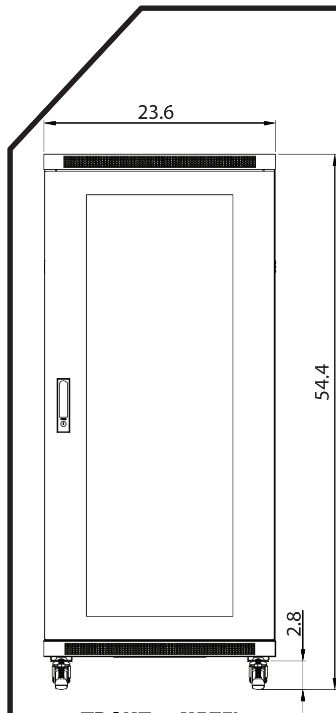
FRONT VIEW
