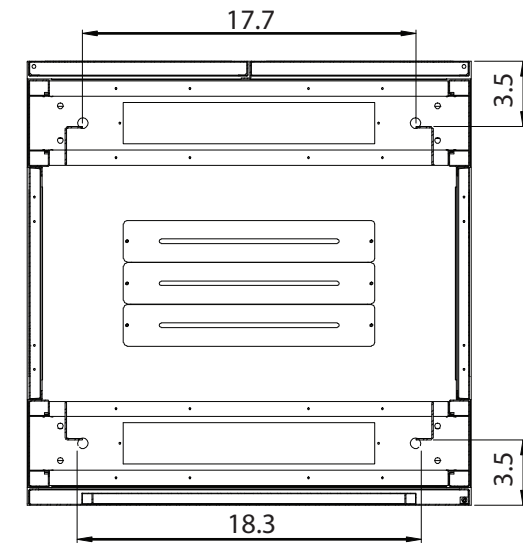
CUT-OPEN VIEW
