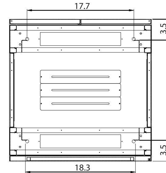
CUT-OPEN VIEW
